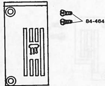
Needle plate (3 Needles)
