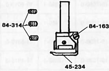
Needle holder (2,3 Needles)
