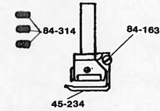
Needle holder (2,3 Needles)
